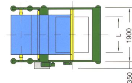
Vista in pianta - Plant view Vista en planta - Grundriss. Ansicht
